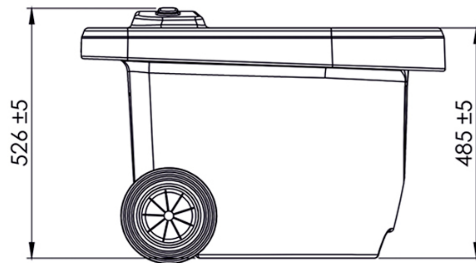
SIDE
