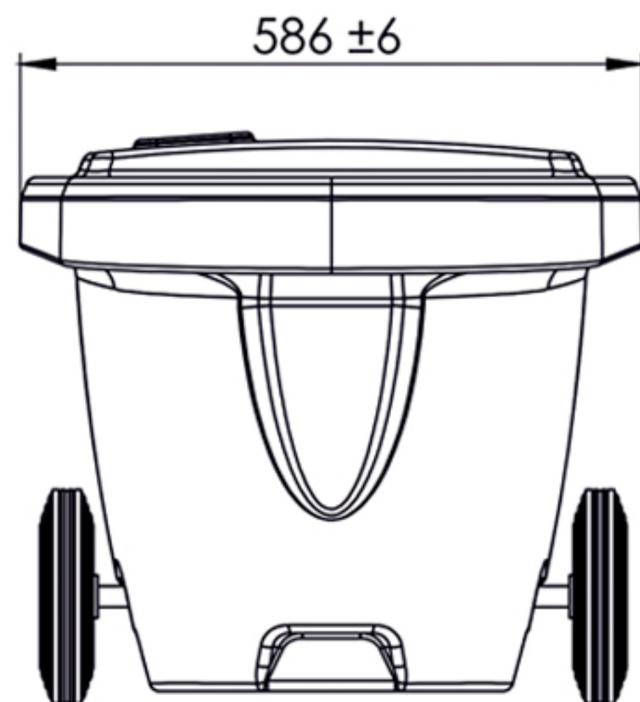
FRONT
